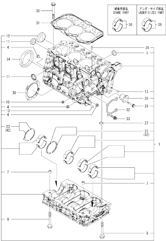
OCD50-M01130 3TNM74F-SAAY Fig.1. CYLINDER BLOCK
