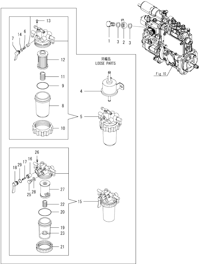
Fig.13. FUEL PIPE
